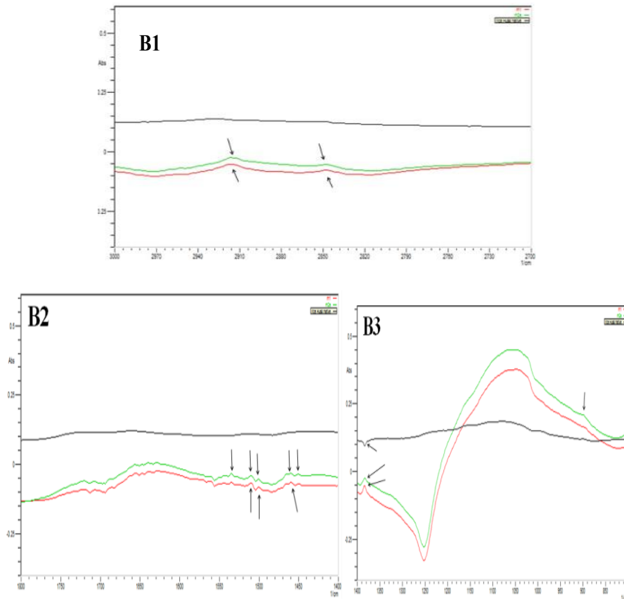
Fig. 1. B (B1- B3) - Overlapped view of FTIR spectra of native RH (black online), 2% HNO 3 pretreated RH (red online) and 10% HNO 3 pretreated RH (green online)
