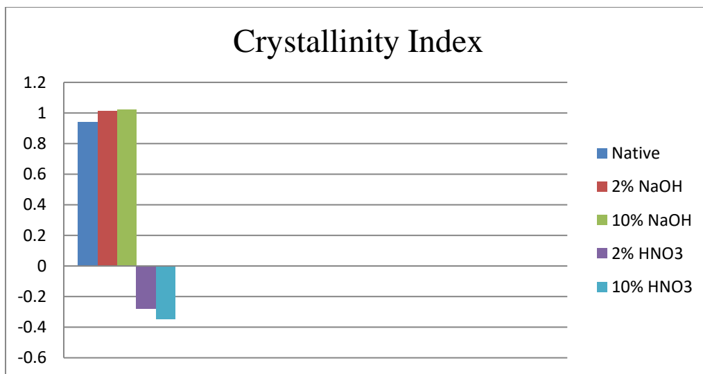
Fig. 2. Total crystallinity index of native and pretreated rice husk
