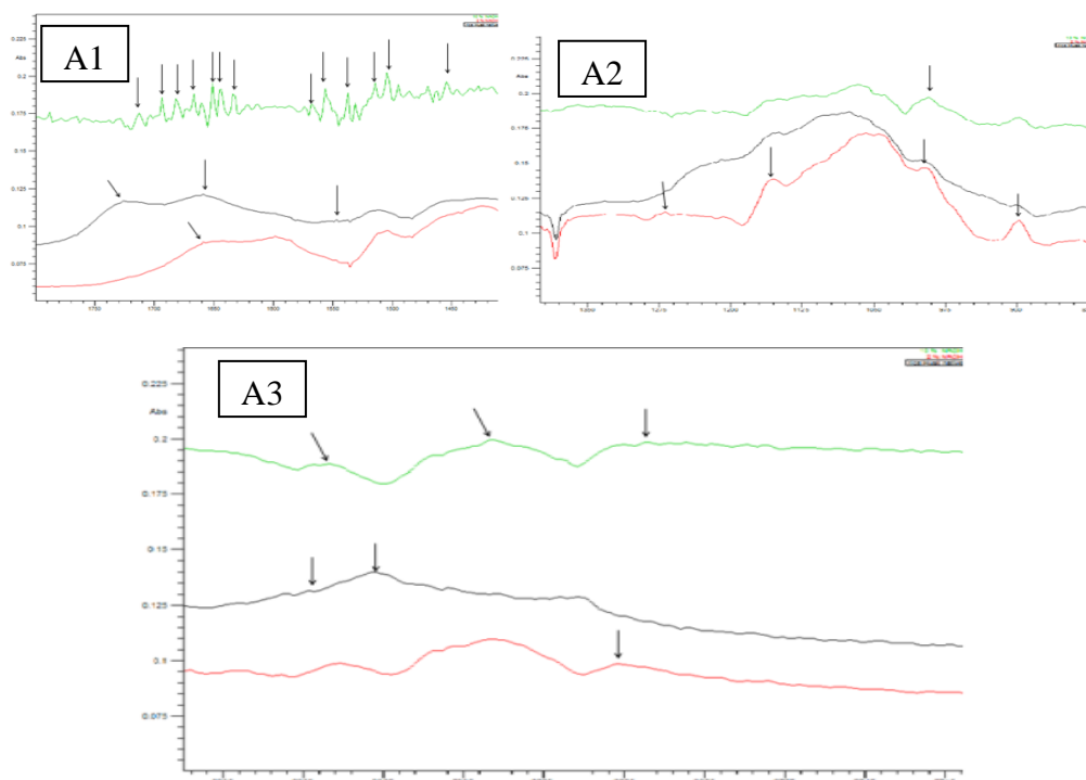
Fig. 1. A (A1-A3) - Overlapped view of FTIR spectra of native RH (black online), 2% NaOH pretreated RH (red online) and 10% NaOH pretreated RH (green online)
