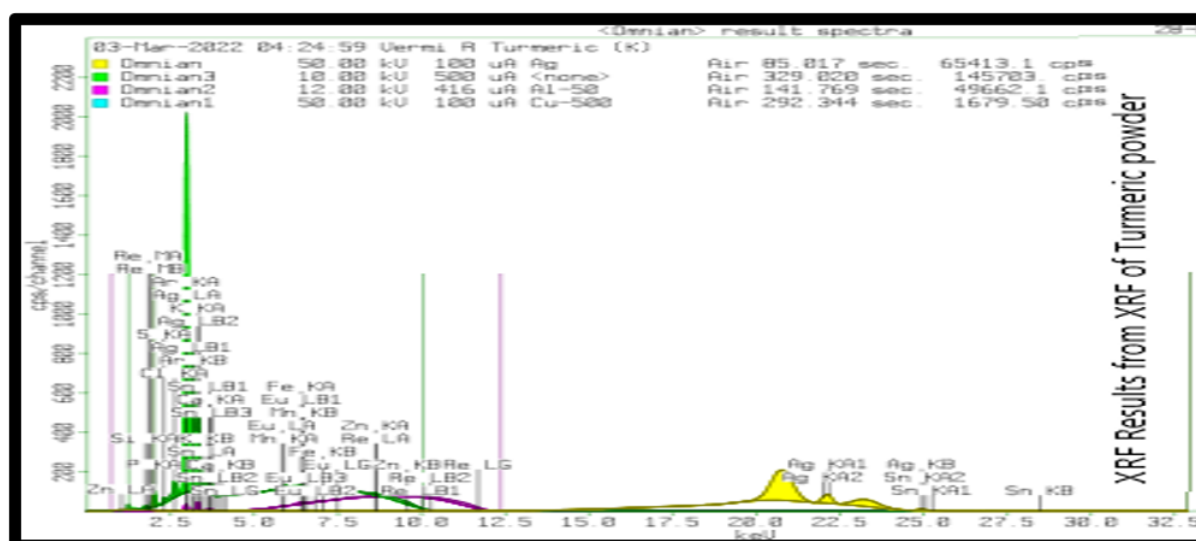
Fig. 4. Elements, compounds in yellow /black turmeric tested under X-RF Spectrometer
