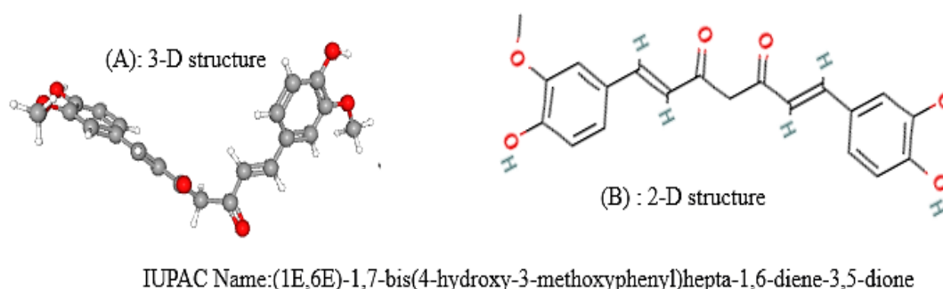
Fig. 2. The 2-D (B) and 3-D (A) structure of turmeric (Curcumin) as per IUPAC
